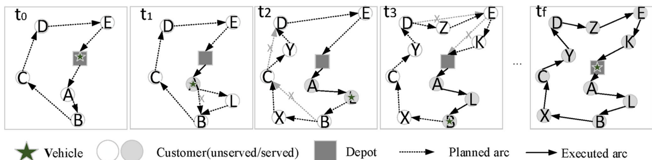
Fig. 1 Illustration of the DU-VRP
