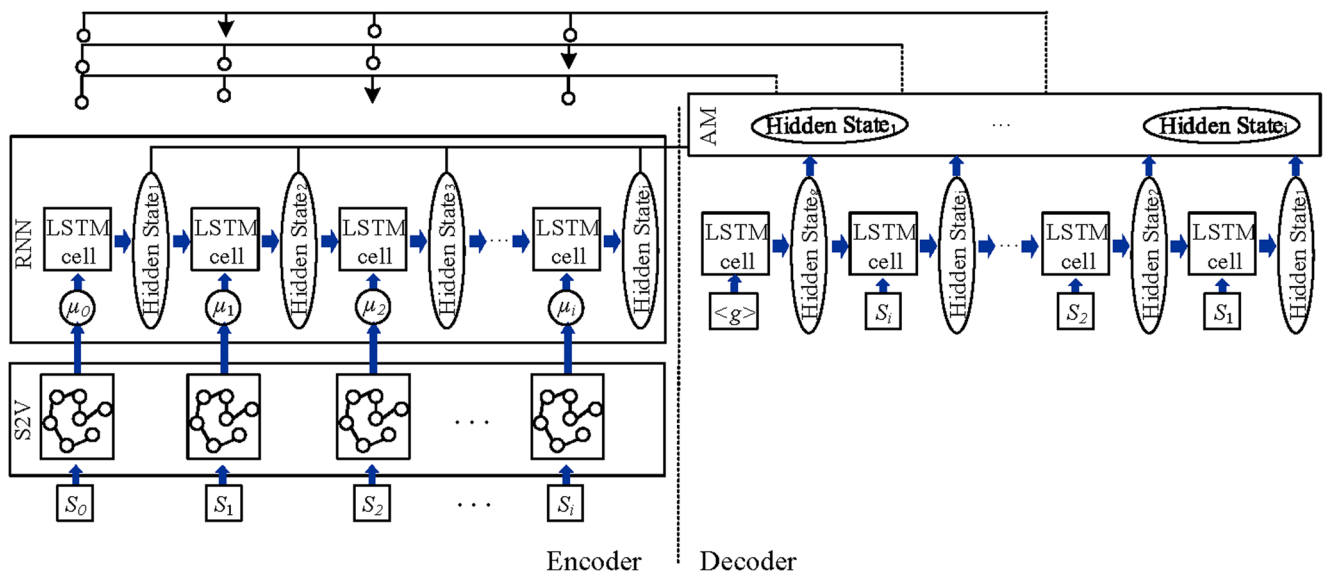
Fig. 6 The process of an improved neural network for the DU-VRP
