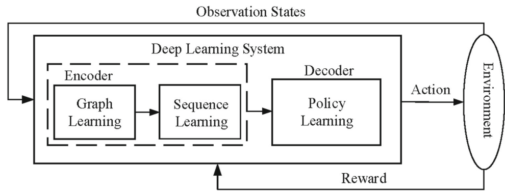
Fig. 7 Interaction agent-environment in the reinforcement learning for the DU-VRP
