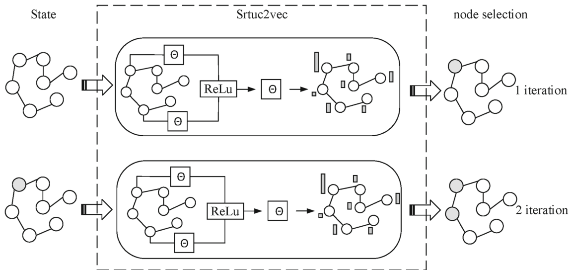
Fig. 5 The process of the input layer in the deep learning for the DU-VRP
