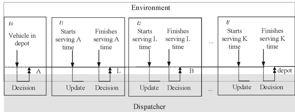
Fig. 2 Timeline of events for the DU-VRP
