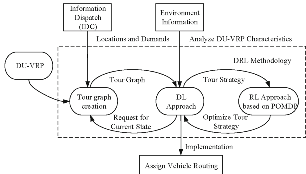
Fig. 4 The structure of the DRL methodology for the DU-VRP
